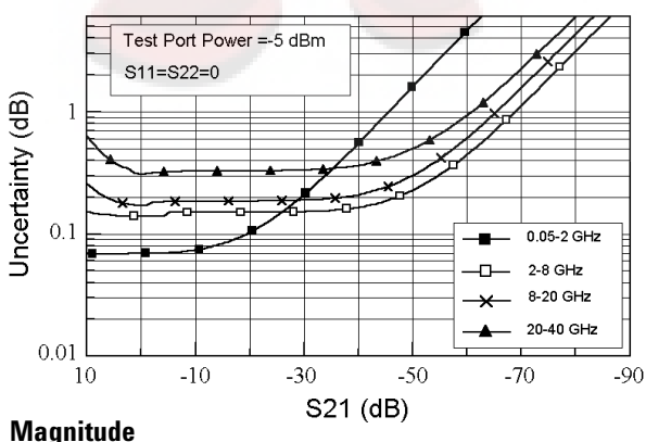
8722D OPT 007/085 with 85056A Calibration Kit
